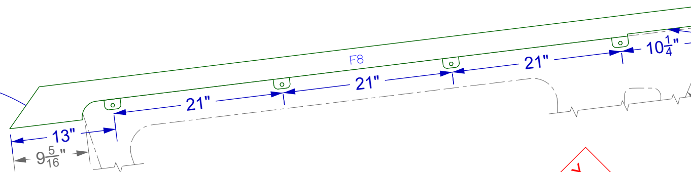
F8 STBD FWD TRANSV. FASCIA - REMOVABLE (TABS) OUTWARD-FACING SIDE SHOWN
