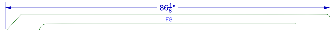
F8 STBD FWD TRANSV. FASCIA - REMOVABLE (TABS)
